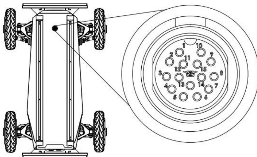
Figure 4-4 Power supply and communication wires
